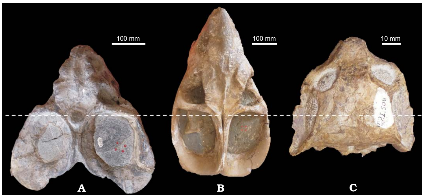
Fig. 4. Skulls of Dicynodontia illustrating the great variability of the shape and size of parietal foramen in Therapsida. A. Large and circular parietal foramen, with a pineal boss in Rachiocephalus , RC 95, Deredrif, Adendorp, South Africa, Cistecephalus–Tropidostoma AZ, 260–255 Ma. B. Slit-like parietal foramen in Dinanomodon , RC09, Stylkrans, South Africa, Cistecephalus AZ, 250–255 Ma. C. Absent foramen in Cistecephalus , BPI/1/506, Towerwater, Murraysburg, South Africa, Cistecephalus AZ, 250–255 Ma.
