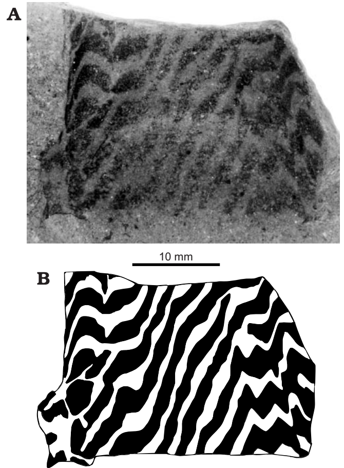
Fig. 1. Adapertural part of orthoceratoid body chamber with preserved colour pattern; counterpart, specimen NM-L 38470. Koněprusy, Klonk section, Lower Devonian, Lochkovian, Lochkov Formation, Monograptus uniformis Zone, probably interbed 20/21 (see Chlupáč et al. 1972). A. Photograph. B. Schematic drawing.
