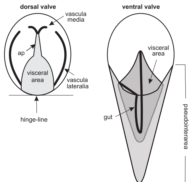
Fig. 3. Schematic reconstruction of lingulotretid brachiopod Lingulosacculus nuda gen. et sp. nov. Abbreviation: ap, anterior projection.
