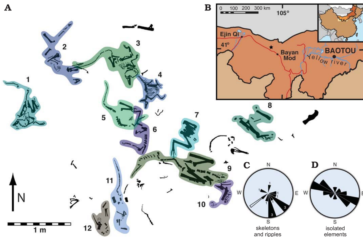
Fig. 1. Suhongtu site, partial quarry map, locality map, and orientation data. A. Map of the central and northern portions of site showing the position of 12 of 13 skeletons. Skeletons 3 and 4 enlarged in Fig. 3. B. Fossil locality ( 41^{\circ}17'10''\text{N} , 103^{\circ}52'38''\text{E} ) located 90 km northwest of Bayan Mod, Inner Mongolia, China. C. Rose-diagram showing trends for skeletons (black, numbers denote skeleton count) and ripples (white). D. Mirror rose-diagram of elongated, isolated elements ( n = 13 ). Trends of skeletons have a strong, non-random ( p < 0.002 ) alignment to southeast. Flow direction of ripples is roughly perpendicular to that of elongate elements.
