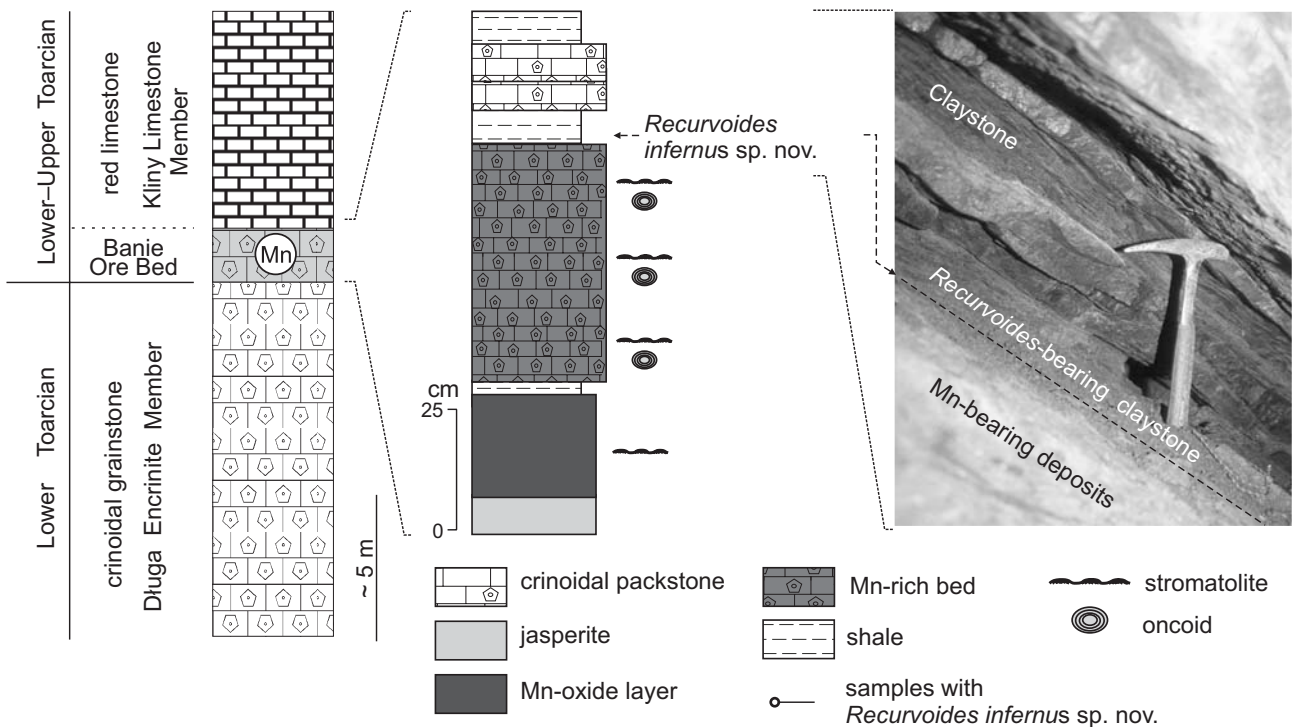
Fig. 2. A. Lithostratigraphic log of the Lower–Middle Jurassic rocks of the Kriżna unit in the Western Tatra Mountains (after Lefeld et al. 1985). B. Lithological sections of the Mn-bearing sequence at the Huciański Klin crest and a photograph from the adit no. 4 described in detail in Jach (2002).
