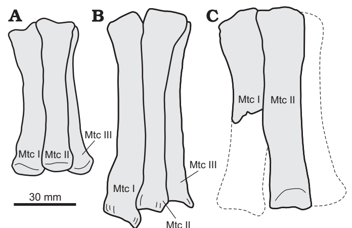
Fig. 10. Metacarpal bones of three ornithomimid taxa shown in articulation. A. Anserimimus planinychus (Upper Cretaceous Nemegt Formation; after Kobayashi and Barsbold 2006; drawing flipped horizontally). B. Ornithomimus edmontonicus (Upper Cretaceous Horseshoe Canyon Formation; after Parks 1933). C. ZPAL MgD-I/65 (Upper Cretaceous Nemegt Formation; this paper). Abbreviation: Mtc, metacarpal.
