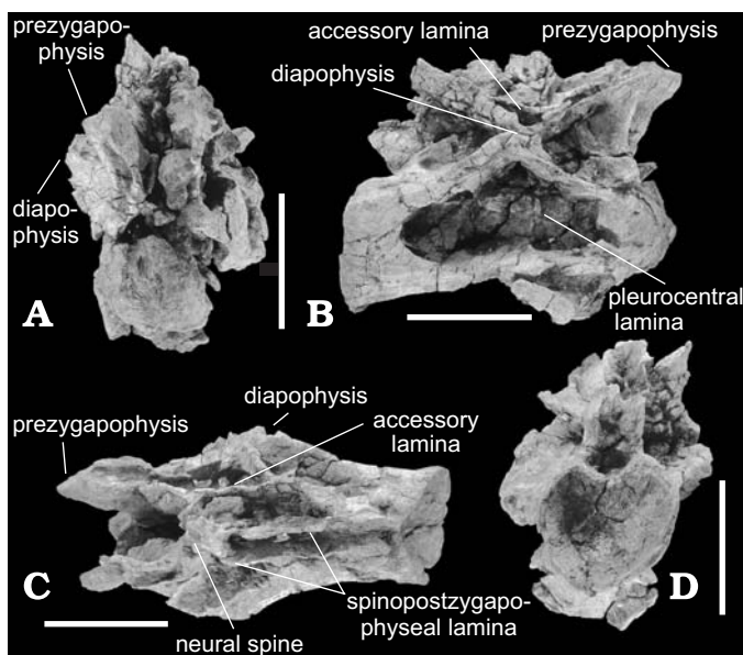
Fig. 6. Anterior-middle cervical vertebra of rebbachisaurid sauropod Demandasaurus darwini gen. et sp. nov. from Late Barremian–Early Aptian, Early Cretaceous of Tenadas de los Vallejos II, Spain, MDS-RVII,589, in anterior (A), right lateral (B), dorsal (C), and posterior (D) views. Scale bars 10 cm.
