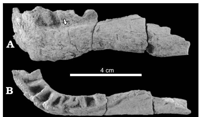
Fig. 3. Left dentary of rebbachisaurid sauropod Demandasaurus darwini gen. et sp. nov. from Late Barremian–Early Aptian, Early Cretaceous of Tenadas de los Vallejos II, Spain, MDS-RVII,443, in lateral (A) and dorsal (B) views. The arrow indicates a depressed area in a dorsolateral position.
