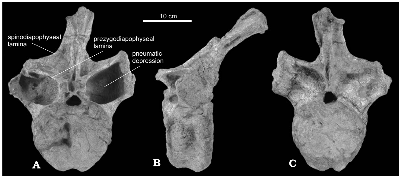
Fig. 11. Anterior caudal vertebra of rebbachisaurid sauropod Demandasaurus darwini gen. et sp. nov. from Late Barremian–Early Aptian, Early Cretaceous of Tenadas de los Vallejos II, Spain, MDS-RVII,610, in anterior (A), lateral (B), and posterior (C) views. The neural spine is incomplete.
