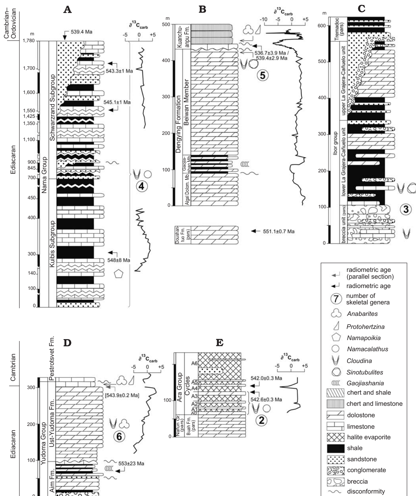
Fig. 2. Stratigraphic distribution of Ediacaran skeletal fossil assemblages from around the world. A. Zaris (Kuibis Subgroup) and Witputs (Schwarzsand Subgroup) subbasins, Nama Basin, Namibia (Grotzinger et al. 1995, 2000, 2005; Saylor et al. 1998; Wood et al. 2002). B. Yangtze Platform, southern Shaanxi, China (Hua et al. 2000b; Steiner et al. 2007; Zhu et al. 2007: lower C isotope curve; Ishikawa et al. 2008: upper C isotope curve; Pb/U radiometric data after Condon et al. 2005; Compston et al. 2008; Zhu et al. 2009). C. Abenójar (Abenójar Village and Tirteafuera River) Anticline, East Lusitanian–Alcudian Zone, central Spain (Ortega Girones and Sánchez Vizcaíno 1987). D. Yudoma River, Uchur-Maya region, Siberian Platform, Russia (C isotope data after Brasier et al. 1994; Podkovyrov and Davydov 1998; Pb–Pb radiometric data after Semikhatov et al. 2003). E. South Oman Salt Basin (Brasier et al. 2000; Amthor et al. 2003; Schröder and Grotzinger 2007). Abbreviations: Dolom., dolomite; Fm., formation; Gr., group; Mb., member.
