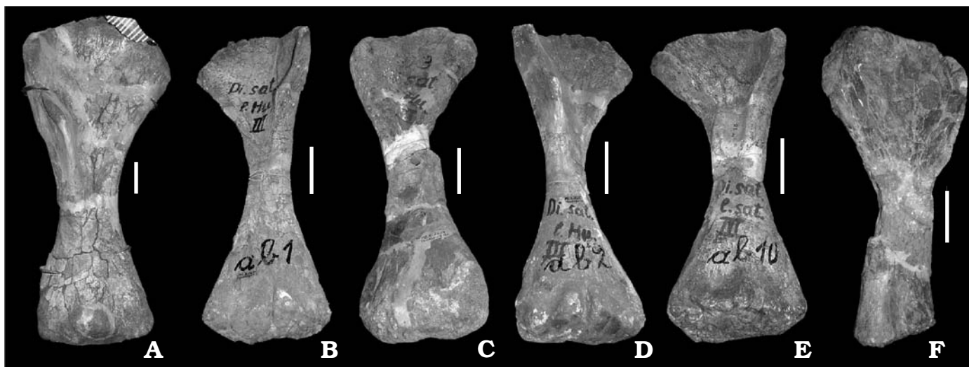
Fig. 2. Studied sample of humeri of dicraeosaurid dinosaurs Dicraeosaurus and Amargasaurus in anterior aspect. Dicraeosaurus hansemanni (A), Dicraeosaurus sattleri (B–E), and Amargasaurus cazau (F). A. MB.R.4912, right humerus. B. MB.R.2631, right humerus. C. MB.R.2634, right humerus. D. MB.R.2655, left humerus. E. MB.R.2657, left humerus. F. MACN-N 15, right humerus. Scale bars 10 cm.
