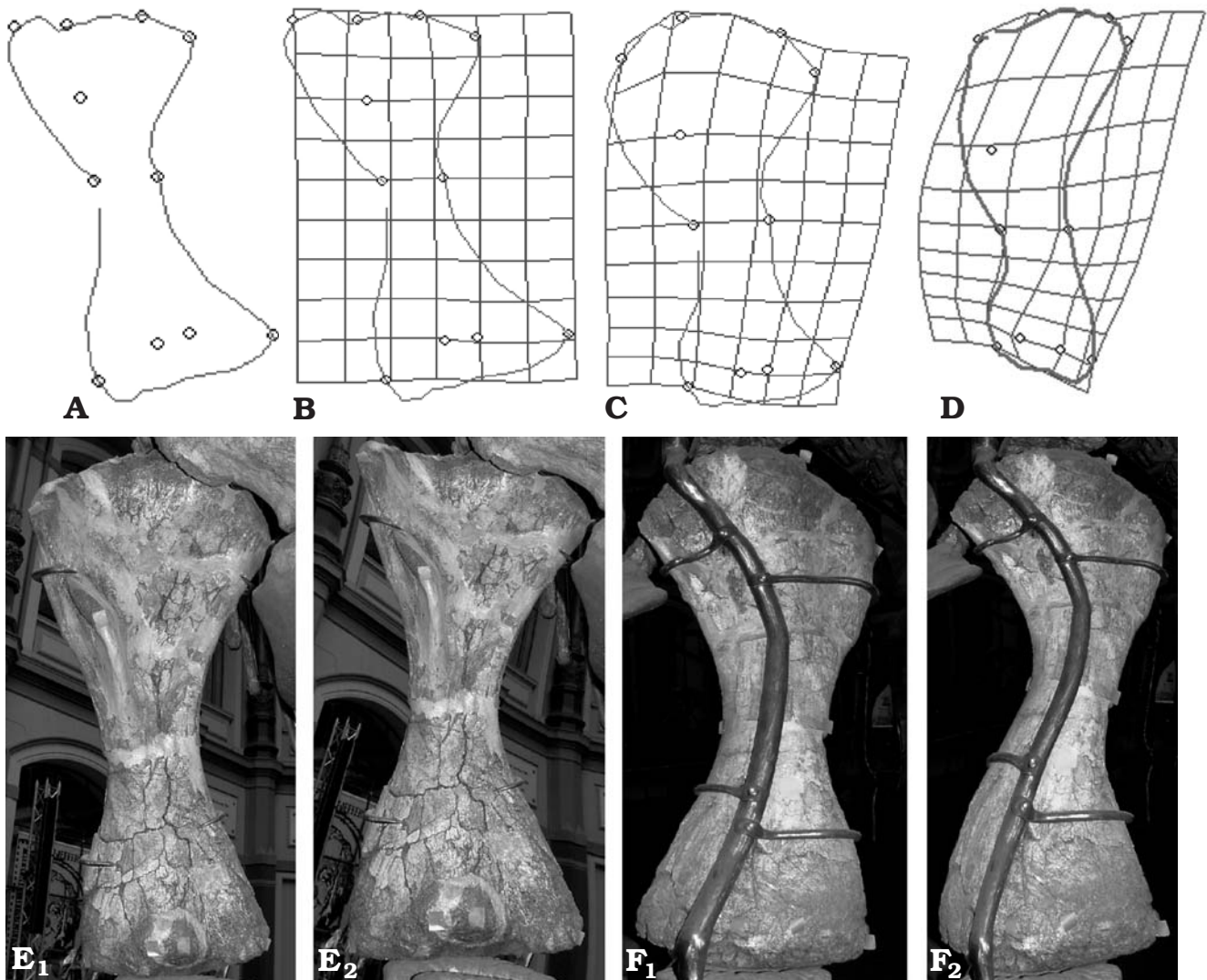
Fig. 5. Thin-plate Splines of humeri of dicraeosaurid dinosaurs Dicraeosaurus and Amargasaurus . A . Reference shape of humeri of Dicraeosaurus sattleri . B . Same reference shape adjusted onto the landmark positions of MB.R.2631 ( Dicraeosaurus sattleri ). C . Same reference shape adjusted onto the landmark positions of MB.R.4912 ( Dicraeosaurus hansemanni ). D . Reference shape of humerus of Amargasaurus cazauui , MACN N-15. Only landmarks are displaced, whereas outlines are left for better overview of shape; printouts from tpsSpln (Rohlf 2004a). E , F . Right humerus MB.R.4912 of D. hansemanni , photograph in comparison with shape-changes when fitted onto reference shape of D. sattleri . Photographs ( E , F ) and shape of anterior ( E ) and posterior ( F ) faces modified by tpsSuper. Not to scale.
