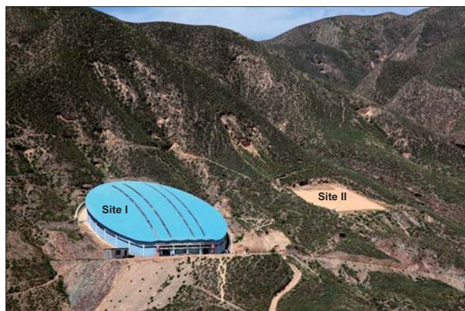
Fig. 1. Photograph of Liujiaxia Dinosaur National Geopark sites I and II.
