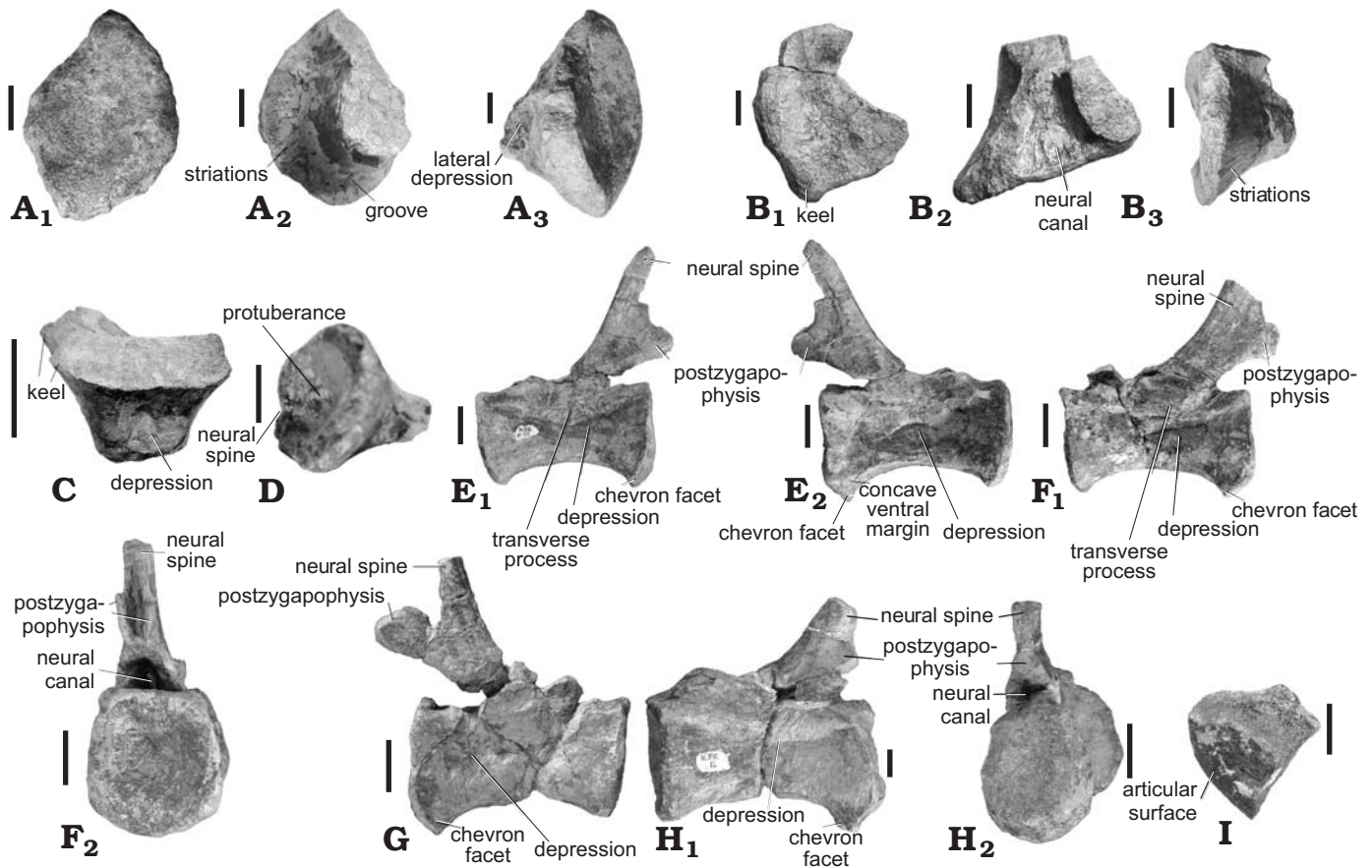
Fig. 7. Ceratosaurian theropod Camarillasaurus cirugedae gen. et sp. nov. from the Camarillas Formation of Camarillas, Soria Province, Spain, caudal vertebrae: A . MPG-KPC19, in ?anterior (A 1 ), ?posterior (A 2 ), and lateral (A 3 ) views. B . MPG-KPC18, in ?anterior (B 1 ), dorsal (B 2 ), and lateral (B 3 ) views. C . MPG-KPC15, in lateral view. D . MPG-KPC46, in ?posterior-lateral view. E . MPG-KPC10, in left lateral (E 1 ) and right lateral (E 2 ) views. F . MPG-KPC11, in left lateral (F 1 ) and posterior (F 2 ) views. G . MPG-KPC13, in left lateral view. H . MPG-KPC12, in left lateral (H 1 ) and posterior (H 2 ) views. I . MPG-KPC22, in ?anterior view. Scale bars A 2 , C–G, H 2 , 20 mm; A 1 , H 1 , 10 mm.
