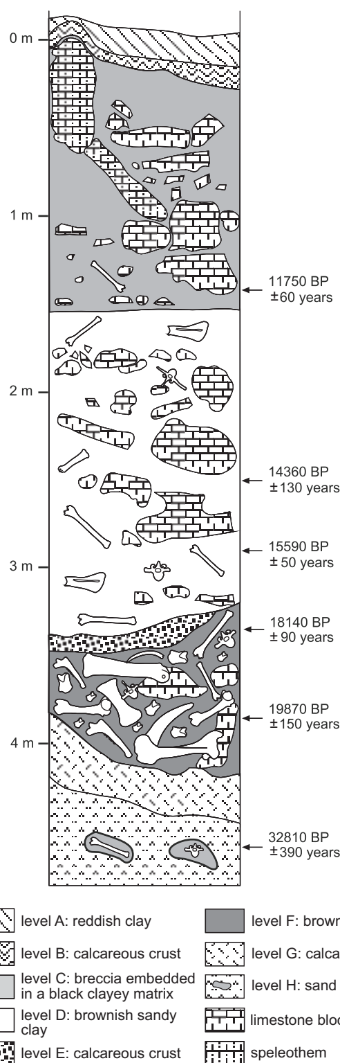
Fig. 2. Stratigraphic section and radiocarbon dates for the locality of Kiputz IX.
