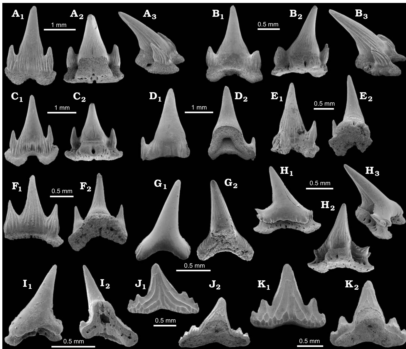
Fig. 8. Carcharhiniiformes from the Danian of Stevns Kridtbrud and Kulstirenden. A–F. “ Scyliorhinus ” elongatus (Davis, 1887). A. MGUH 29861 (Ce) anterior tooth in labial (A 1 ), lingual (A 2 ), and lateral (A 3 ) views. B. MGUH 29862 (Ce) anterior tooth in labial (B 1 ), lingual (B 2 ), and lateral (B 3 ) views. C. MGUH 29863 (Ce) lateral tooth in labial (C 1 ) and lingual (C 2 ) views. D. MGUH 29864 (Ce) lateral tooth in labial (D 1 ) and lingual (D 2 ) views. E. MGUH 29865 (Ce) lateral tooth in labial (E 1 ) and lingual (E 2 ) views. F. MGUH 29866 (Ce) posterior tooth in labial (F 1 ) and lingual (F 2 ) views. G–I. “ Scyliorhinus ” biddlei Halter, 1995. G. MGUH 29867 (Ce) anterior tooth in labial (G 1 ) and lingual (G 2 ) views. H. MGUH 29868 (Ce) lateral tooth in labial (H 1 ), lingual (H 2 ), and lateral (H 3 ) views. I. MGUH 29869 (Br1) lateral tooth in labial (I 1 ) and lingual (I 2 ) views. J, K. Crassescyliorhinus germanicus (Herman, 1982). J. MGUH 29870 (Ce) lateral tooth in labial (J 1 ) and lingual (J 2 ) views. K. MGUH 29871 (Br1) anterior tooth in labial (K 1 ) and lingual (K 2 ) views.
