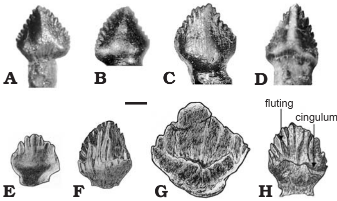
Fig. 4. Teeth of nodosaurid dinosaurs. A–C. Three teeth of the holotype (CEUM 1307) of Gastonia burgei Kirkland, 1998 from Lower Cretaceous of Utah, USA (photographs courtesy of James Kirkland). A. First tooth in ?lingual view. B. Second tooth in ?lingual view. C. Third tooth in ?buccal view. D. Gargoylesaurus parkpinorum Carpenter, Miles, and Cloward, 1998 from the Upper Jurassic of Wyoming, USA (photograph courtesy of K. Carpenter), DMNH 27726, holotype in ?lingual view. E. Unnamed nodosaurid from the Lower Cretaceous of Spain, MPZ 2002/926 in labial view (drawn after Canudo et al. 2004). F. Acanthopholis horridus Huxley, 1867 from the Upper Cretaceous of England, BGS GSM 109045 in ?lingual view (drawn after Pereda-Suberbiola and Barrett 1999). G. Struthiosaurus languedocensis Garcia and Pereda-Suberbiola, 2003 from the Upper Cretaceous of Southern France, UM2 OLV-D18 CV in ?lingual view (drawn after Garcia and Pereda-Suberbiola 2003). H. Edmontonia rugosidens (Gilmore, 1930) from the Upper Cretaceous of USA, NMC 8531 in lingual view (drawn after Barrett 2001). Scale bar: A, B, D, F–H, 3 mm; C, 2 mm; E 1.5 mm.
