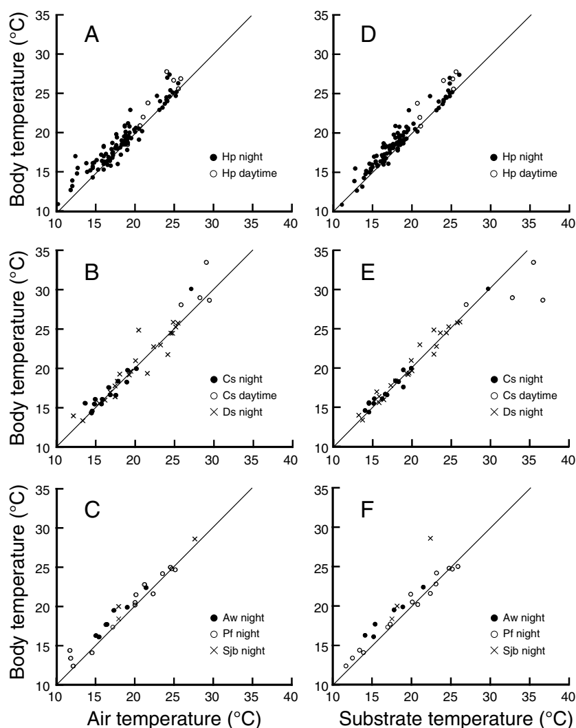
FIG. 1. Thermal relations of six species of snakes observed at night. Relationships between air temperature and body temperature in (A) Hebius pryleri (Hp), (B) Cyclophiopus semicarinatus (Cs) and Dinodon semicarinatus (Ds), and (C) Achalinus wernerii (Aw), Protobothrops flavoviridis (Pf), and Sinomicrurus japonicus boettgeri (Sjb). Relationships between substrate temperature and body temperature in (D) H. pryleri , (E) C. semicarinatus and D. semicarinatus , and (F) A. wernerii , P. flavoviridis , and S. j. boettgeri . For H. pryleri and C. semicarinatus , data measured in the day are also shown. The line where body temperature is equal to ambient temperature is also shown in each figure.
