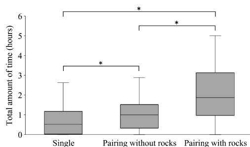
FIG. 2. Total amount of time captive hawksbill turtles spent resting when housed alone ('single') or in pairs in the presence ('pairing with') and absence ('pairing without') of rocks. Whiskers represent the range, boxes represent the inter-quartile range (25–75%), and lines represent the medians. Asterisks represent significant differences among the medians of the total amount of time spent resting ( p < 0.05 ).
