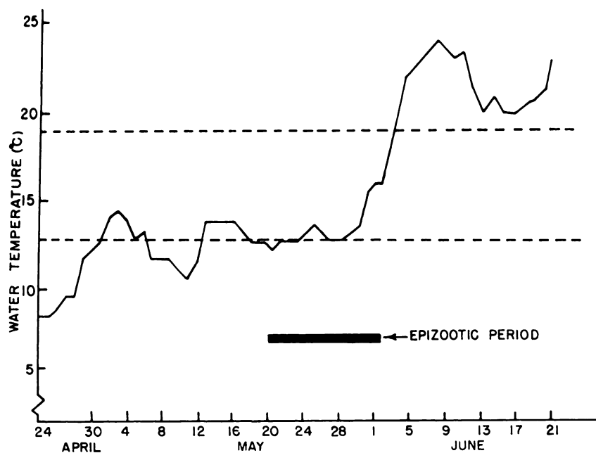
FIGURE 1. Clear Lake water temperatures in relation to furunculosis epizootic, May 1968. Broken lines encompass the optimum temperature range for epizootic outbreak; the broad horizontal line represents the epizootic period.
