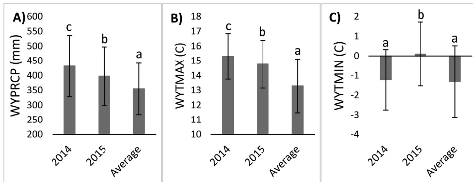
Fig. 6. Study area mean and standard deviation for the 2014, 2015, and 1981–2015 average of A) Water Year Precipitation (WYPRCP), B) Water Year Maximum Temperature (WYTMX), and C) Water Year Minimum Temperature (WYTMIN). Letters indicate significant differences ( p < 0.05 ) among the time period mean climate variable, within each panel (i.e. within each climate variable).
