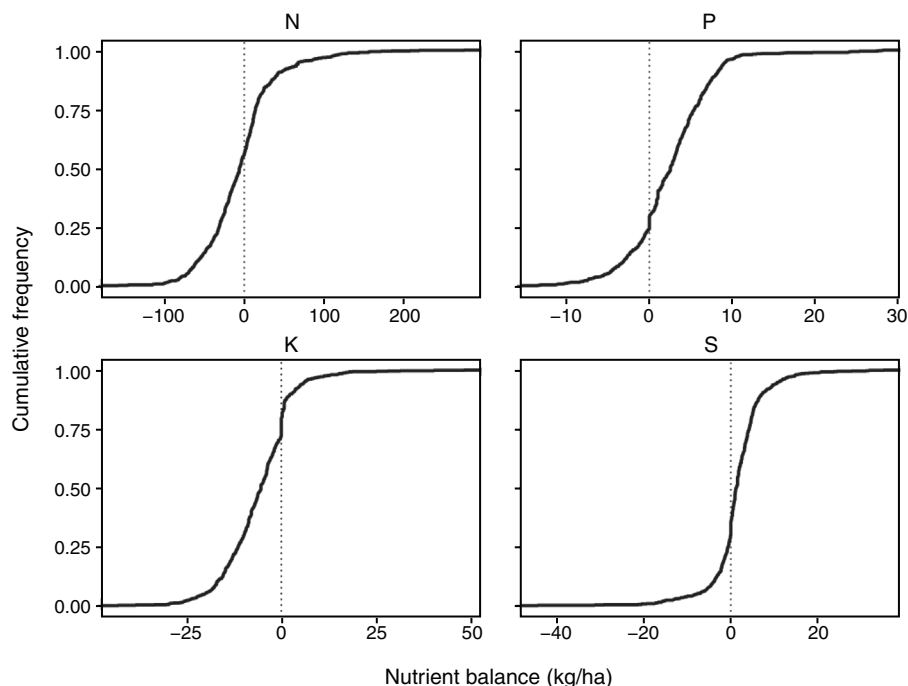
Fig. 7. Cumulative frequency of sequence nutrient balances of N, P, K and S for each paddock, taken from the first year of monitoring (2010 or 2011) to 2014.
