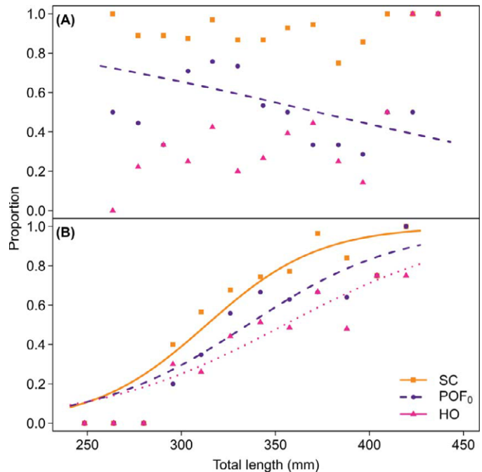
FIGURE 4. Presence or absence of reproductive traits as a function of body size for female Red Porgy sampled in (A) 2008–2009 and (B) 2009–2010. Lines are fitted logistic functions; points are observed proportions (within size-bins) of spawning-capable females (SC), females that possessed day-0 postovulatory follicles (POF 0 ), or females that possessed hydrated oocytes (HO).
