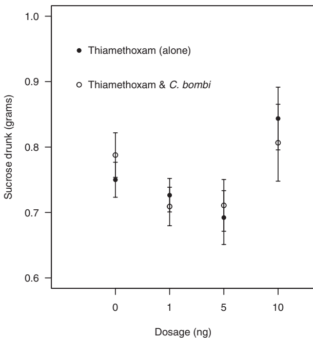
Fig. 3. The mean amount (grams) of sucrose drunk ( \pm SE) over 96 h from parasitized and unparasitized bumblebees ( C. bombi ) acutely exposed to varying dosages of thiamethoxam. Subjects that did not survive the experiments were excluded from this analysis.
