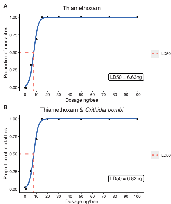
Fig. 1. Dose-dependent plots demonstrating the LD 50 values for bees exposed to thiamethoxam in isolation (A) and bees inoculated with C. bombi and exposed to varying dosage of thiamethoxam (B). We found no difference in the LD 50 between parasitized and unparasitized bees.
