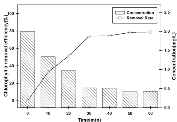
Figure 9. Removal efficiency of chlorophyll a as a function of contact time under the ferrihydrite/calcined oyster shell hybrid process.
