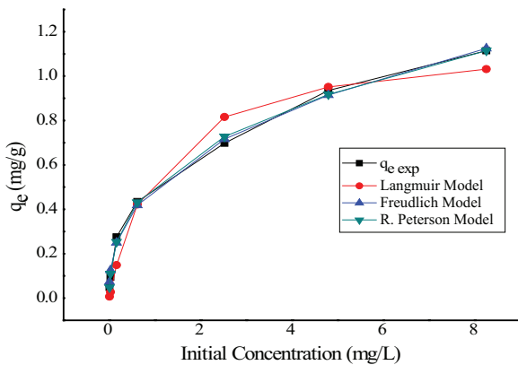
Figure 9. Isotherms of adsorption of phosphate onto pumice.
