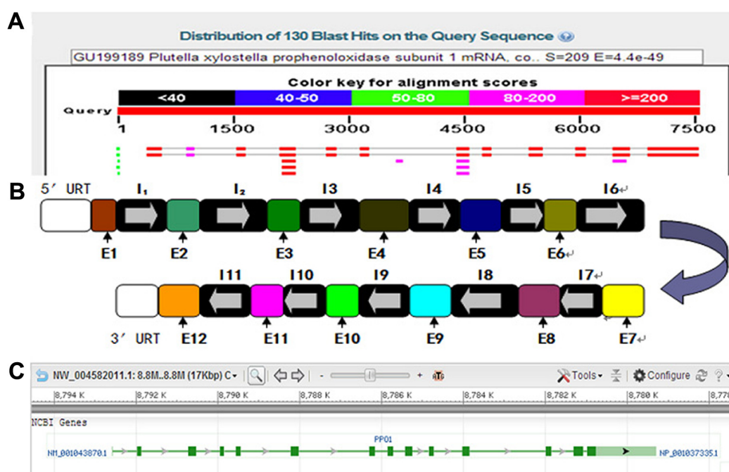
Figure 2. The situation of exons and introns. (A) Sequencing results by BLAST. (B) The schematic arrangement of exons and introns, I 1-11 means the intron I 1-11 ; E 1-12 means the exon E 1-12 . (C) The retrieval results of B. mori PPO1 from NCBI.
