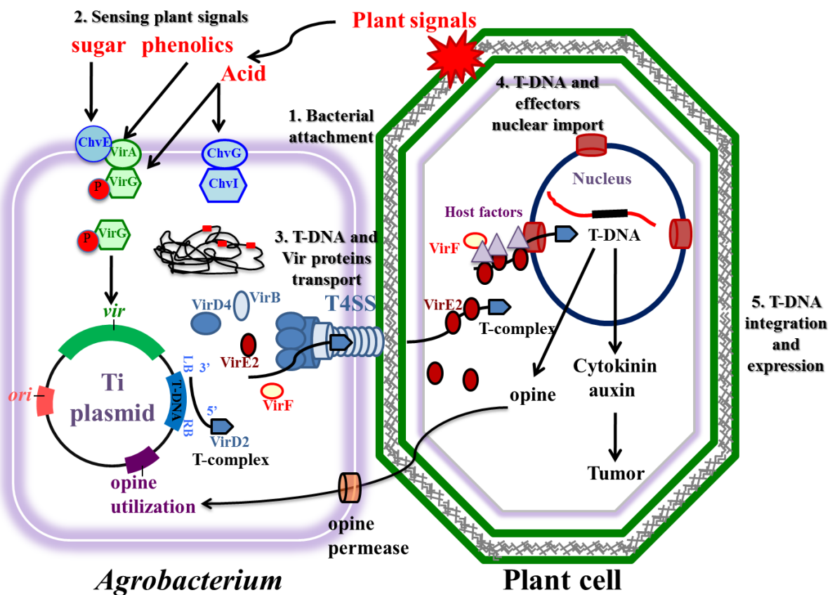
Figure 1. Major steps of the Agrobacterium tumefaciens -mediated plant transformation process.
