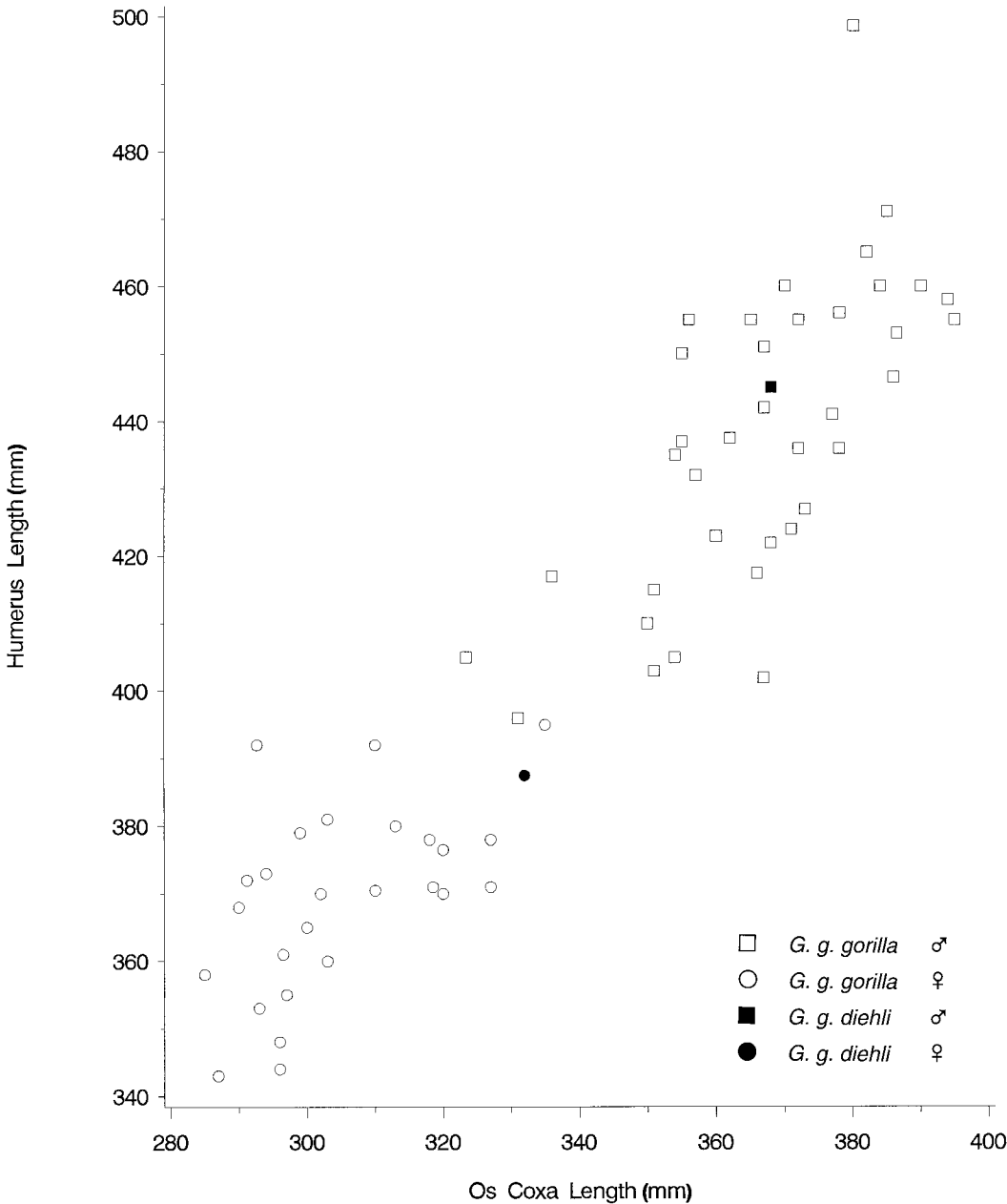
Fig. 12. Plot of humeral length vs. length of os coxa in Cross River gorillas and in non-Cross-River western gorillas. Least square regression of the non-Cross-River gorilla datum points fits a line with a slope = 1.003, y' = 68.03 , adjusted R^2 = 0.83 .
