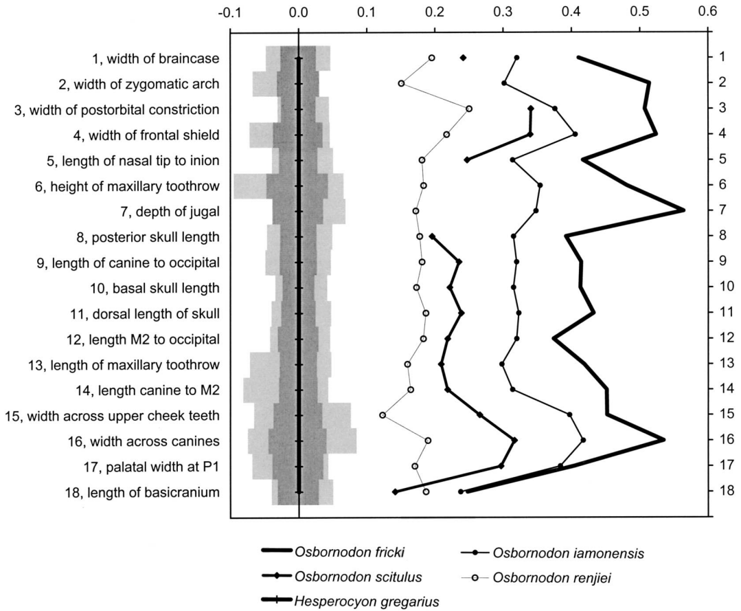
Fig. 8.4. Log-ratio diagram (sensu Simpson, 1941) of cranial measurements for species of Osbornodon , using Hesperocyon gregarius as standard (straight line at zero axis). See Wang (1994) for definitions of measurements and data on other species of Osbornodon . Darkly shaded bars represent one standard deviation above and below the means and lightly shaded bars represent upper and lower ranges for Hesperocyon gregarius .
