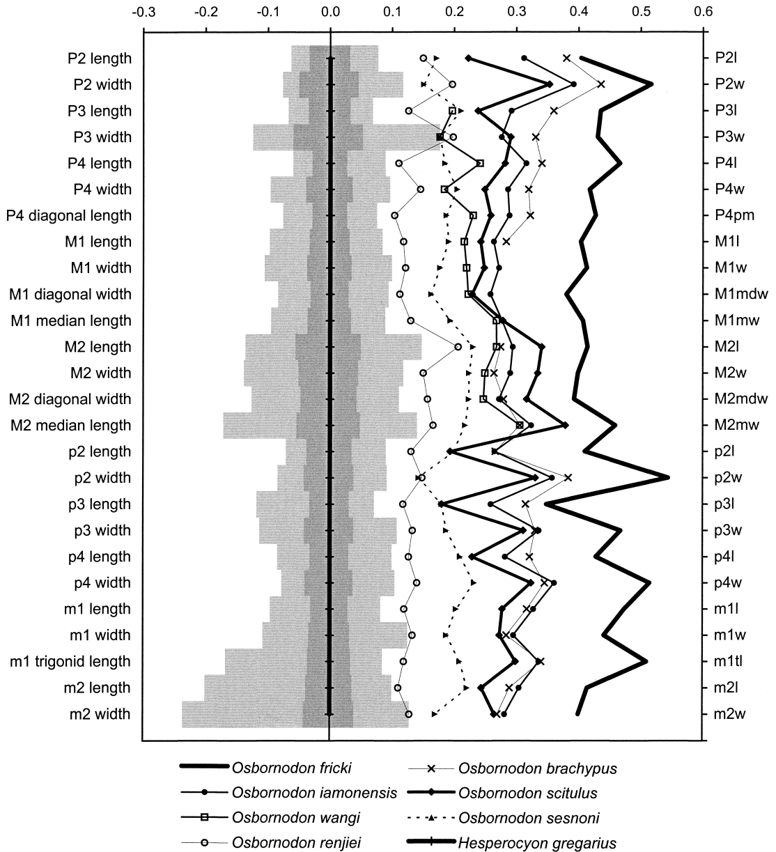
Fig. 8.5. Log-ratio diagram (sensu Simpson, 1941) of dental measurements for species of Osbornodon , using Hesperocyon gregarius as standard (straight line at zero axis). See tables 8.1 and 8.2 for dental measurements of O. scitulus and Wang (1994) for definitions of measurements and data on other species of Osbornodon . Darkly shaded bars represent one standard deviation above and below the means and lightly shaded bars represent upper and lower ranges for Hesperocyon gregarius .
