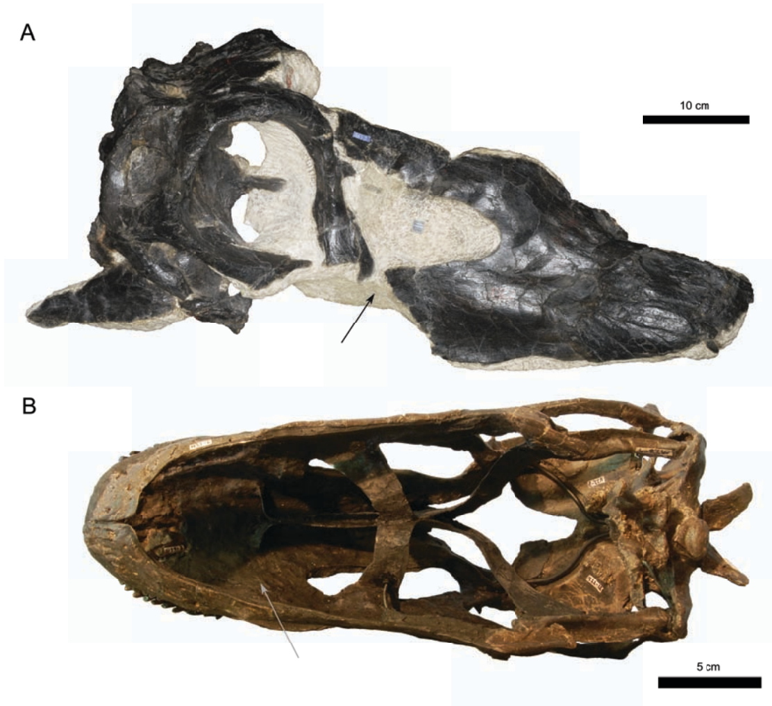
FIGURE 1. Usual preservation of diplodocid skulls. A. Galeamopus pabsti USNM V 2673 (right lateral view) is preserved on a slab of matrix (black arrow). B. Kaatedocus siberi SMA 0004 (ventral view) is mounted on a metal structure mimicking the palatal complex, which is fixed onto the medial side of the facial bones (black elements in center of image, and gray arrow). Photographs by M. Eklund (A) and E. Tschopp (B).
