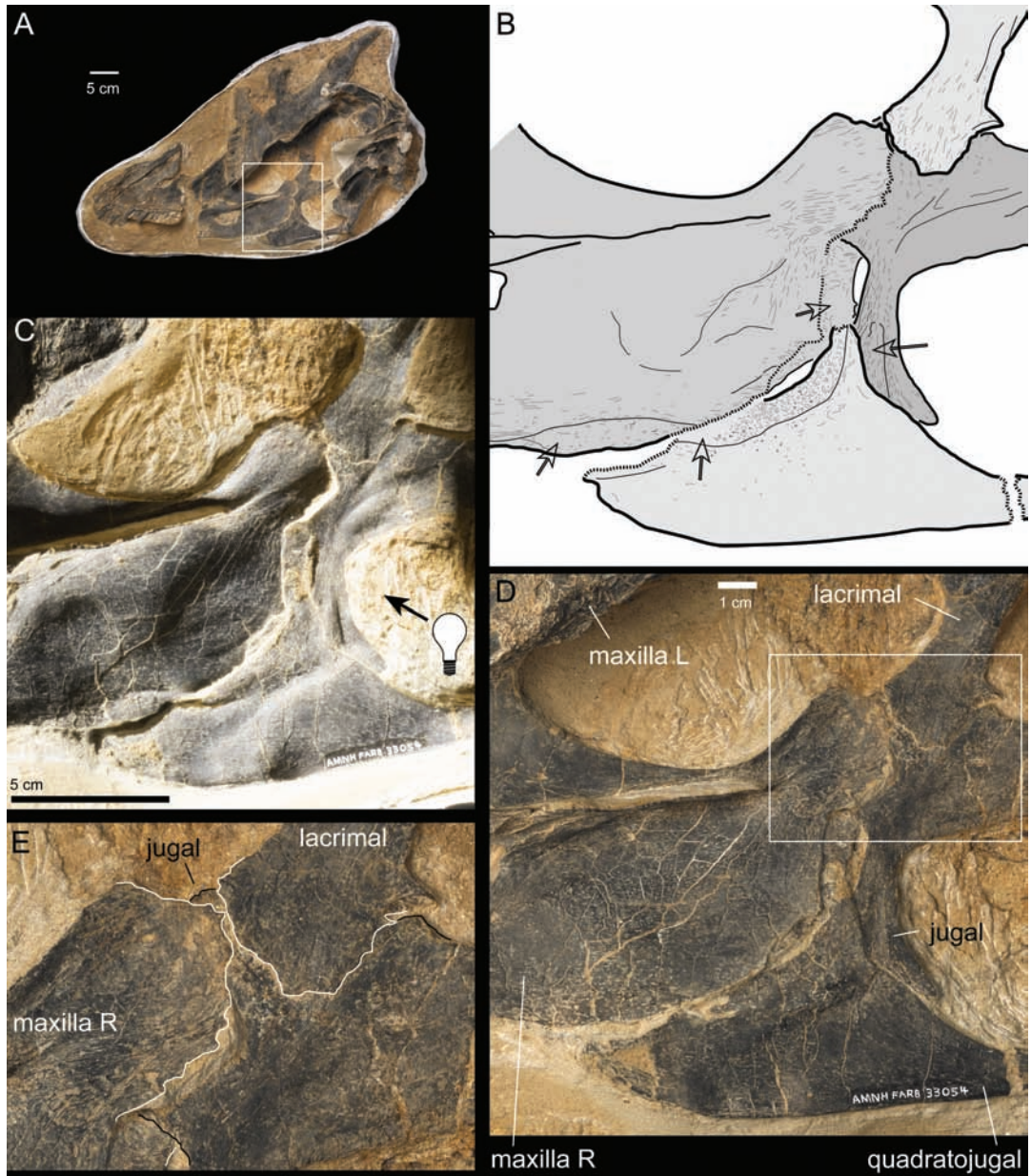
FIGURE 3. Overlapping joints in the diplodocid skull AMNH FARB 33054. A. Overview of the entire skull. B. Drawing of the overlapping joints between the maxilla, quadratojugal, jugal, and lacrimal in medial view, traced from photograph in D. Articular facets indicated with arrows. C. Photograph under oblique lighting (light source located at the bottom right, see icon) to highlight subtle ridges delimiting the facets on the maxilla, quadratojugal, and jugal. D. Photograph under usual lighting, indicating the visible bones; white rectangular indicates area enlarged in E. E. Detail of overlapping joints between maxilla, jugal, and lacrimal, showing the contribution of the jugal in the margin of the antorbital fenestra on the lateral surface of the skull. White (maxilla and lacrimal) and black (jugal) lines highlight the margins of the bones as preserved. Photographs by M. Ellison (A, D, E) and M. Eklund (C).
