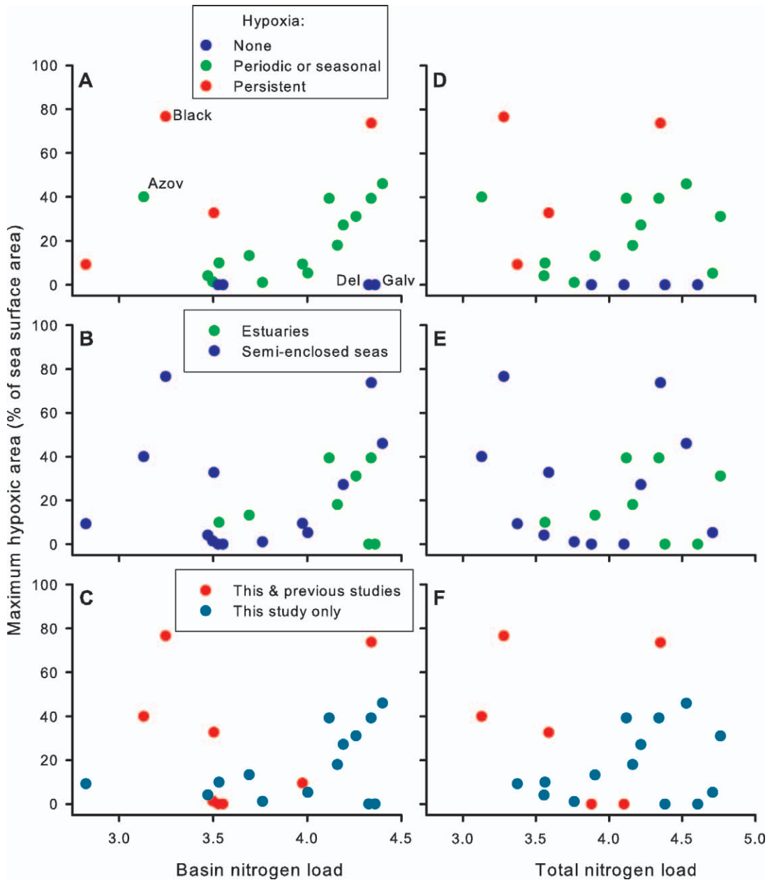
FIGURE 2.—Relationships between maximum spatial extent of hypoxia (area with dissolved oxygen < 3 mg/L expressed as a percentage of system surface area) and nitrogen loading ( \log_{10} [kg/km 2 of sea surface per year]) from watershed sources only (“basin” nitrogen loads; left-hand panels) and estimates of total nitrogen loads that include inputs from downstream or oceanic sources (right-hand panels). Different colors distinguish systems according to (A, D) the frequency and/or duration of hypoxia, (B, E) system type or size, and (C, F) inclusion in previous cross-system analyses. Abbreviations are as follows: Black = Black Sea, Azov = Sea of Azov, Del = Delaware Bay, and Galv = Galveston Bay.
