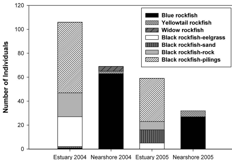
FIGURE 3.—Rockfish species composition in estuarine and nearshore sampling sites along the central Oregon coast during 2004 and 2005. For estuary sites, the proportional distribution of black rockfish within eelgrass, rock, piling, and sand habitats is shown.
