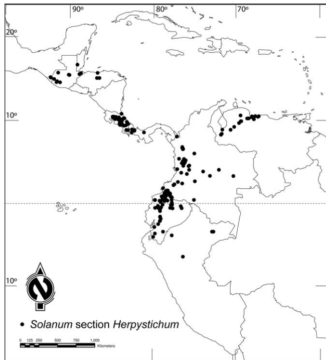
FIG. 3. Distribution of Solanum sect. Herpystichum .
