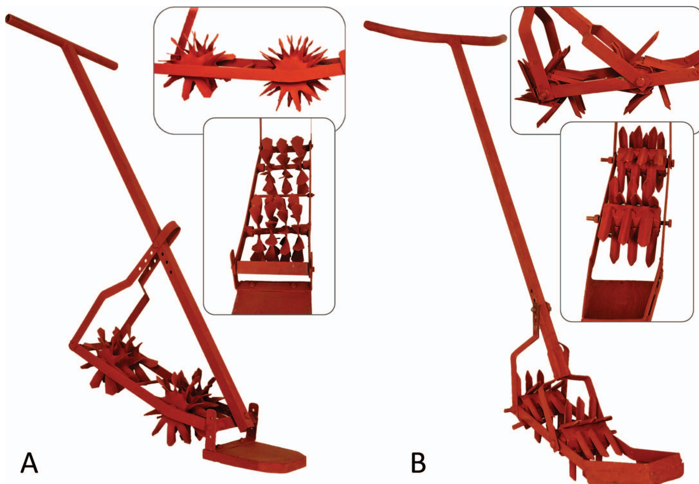
Figure 1. View of the twisted-spike floating weeder, with details of the weeder drum in the right-hand upper corner (A) and the straight-spike floating weeder, with details of the weeder drum in the right-hand upper corner (B). Source: AfricaRice. (Color for this figure is available in the online version of this article.)
