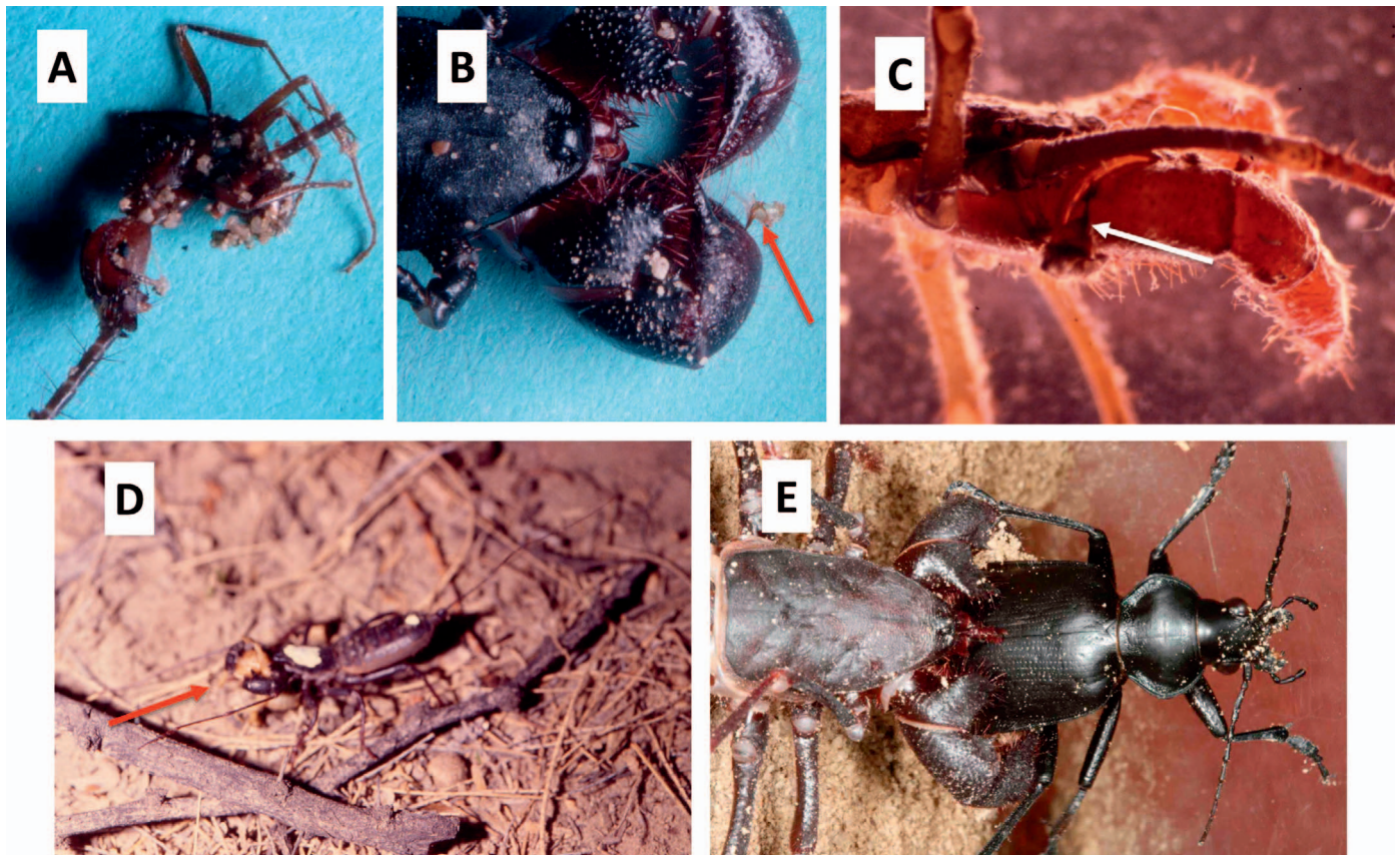
Figure 2.—Vinegaroons in captivity and in the field with different prey items. (A) A still-attached dead harvester ant, Pogonomyrmex maricopa , that had bitten and severed the tail of a vinegaroon. (B) Autotomized stinger of a Pogonomyrmex maricopa (red arrow) remaining attached in the intersegmental membrane of the pedipalp of a 3 rd instar vinegaroon that was killed by the sting. (C) Autotomized stinger of a Pogonomyrmex maricopa (white arrow) remaining attached in the intersegmental membrane of the pedipalp of a 1 st instar vinegaroon that was killed by the sting. (D) A vinegaroon consuming an unidentified prey (red arrow) in the study site. (E) A vinegaroon attempting to penetrate the hard exoskeleton of a beetle, Calosoma sp. Vinegaroons often held these beetles for several hours while attempting to subdue them before finally succeeding.
