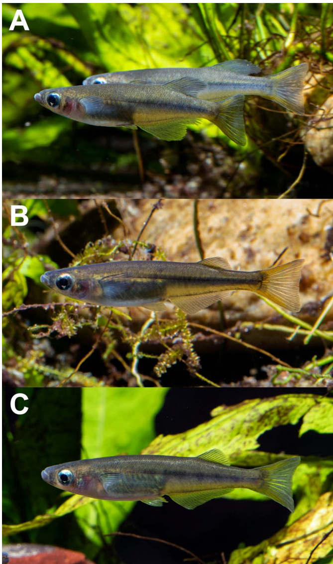
Fig. 3. Life coloration of fish from the type locality under aquarium conditions (uncatalogued specimens). (A) Two males in normal coloration. (B) Female in normal coloration. (C) Female faintly showing the distinctive blotches along the lateral line.
