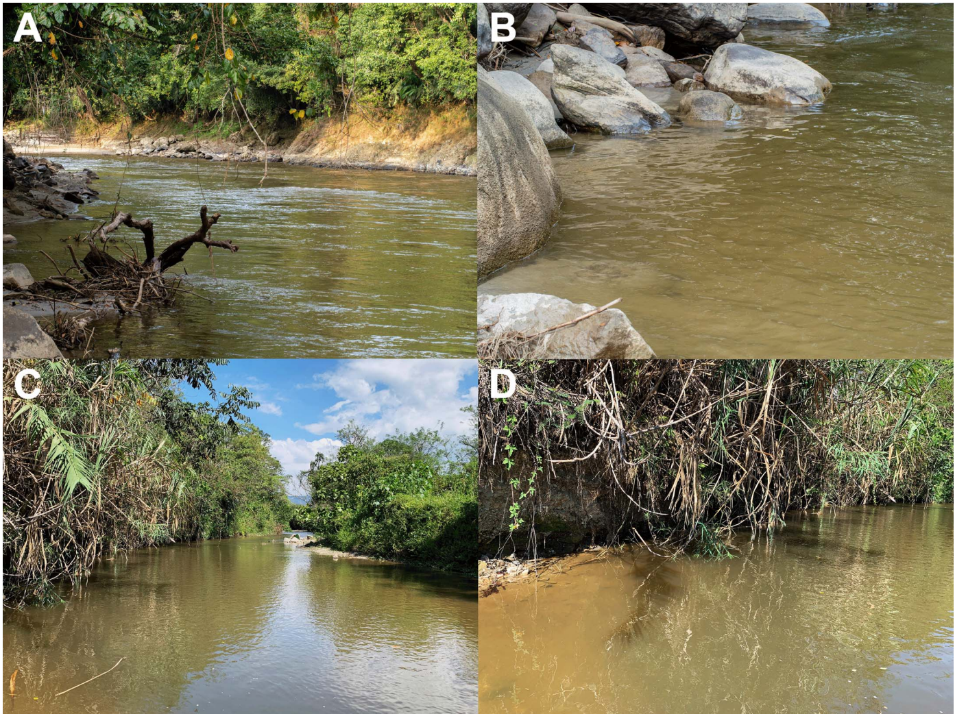
Fig. 6. Habitat at collection localities. (A, B) Type locality at Lariang River near Lengkeka Village, Bada Valley, Poso Regency, Central Sulawesi; (C, D) Pambungu River near Watutau Village in Napu Valley, Poso Regency, Central Sulawesi. (B) and (C) depict microhabitats in which O. polylepis was collected. (Photographs A and B by M. Mejía Estrada.)
