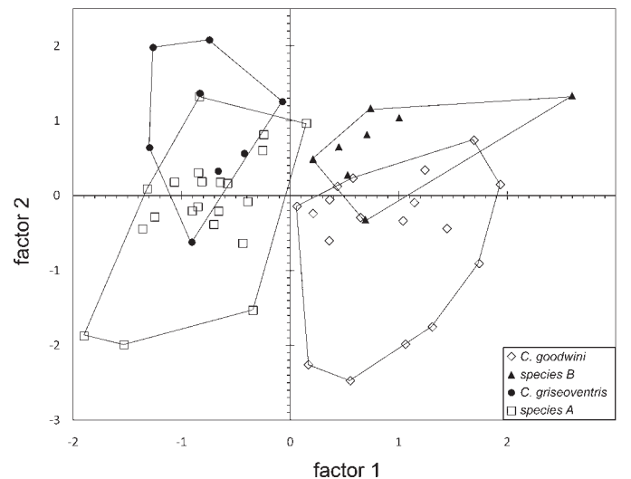
FIG. 2.—Plot of scores on first 2 axes from principal components analysis of skulls of Cryptotis goodwini , C. griseoventris , species A, and species B (see Table 3).
