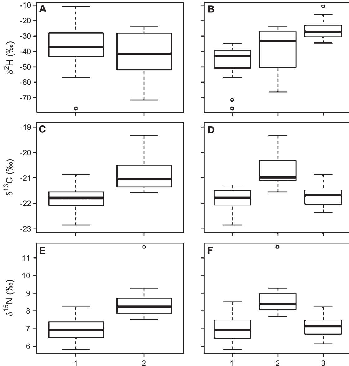
FIGURE 1. Variation in claw stable isotopes of hydrogen ( \delta^2\text{H} : A, B ), carbon ( \delta^{13}\text{C} : C, D ), and nitrogen ( \delta^{15}\text{N} : E, F ) in Vaux's Swifts from a roost site on Vancouver Island, British Columbia, Canada. Claws were clustered into 2 ( A, C, E ) or 3 ( B, D, F ) clusters. The median, interquartile range (IQR), and outliers ( >1.5 \times \text{IQR} ) are shown.
