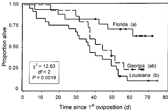
Fig. 2. Survivorship curves for three populations, beginning at first oviposition. Open points on the curves represent one or more censored observations. Overall \chi^2 is for a nonparametric log-rank test of the null hypothesis of equivalent survivorship curves for FL ( N = 18 ), GA ( N = 15 ), and LA ( N = 25 ). Curves associated with the same letters are not significantly different by pairwise log-rank tests ( \alpha = 0.05 ).
