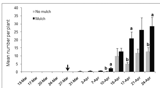
Fig. 1. Mean numbers ( \pm SE) of Microtheca ochroloma per turnip plant in straw mulch and no straw mulch treatments. Arrow indicates the date that adults were released in each treatment plot. Different letters above paired bars for a date indicate significant differences between treatments ( P < 0.05 ).
