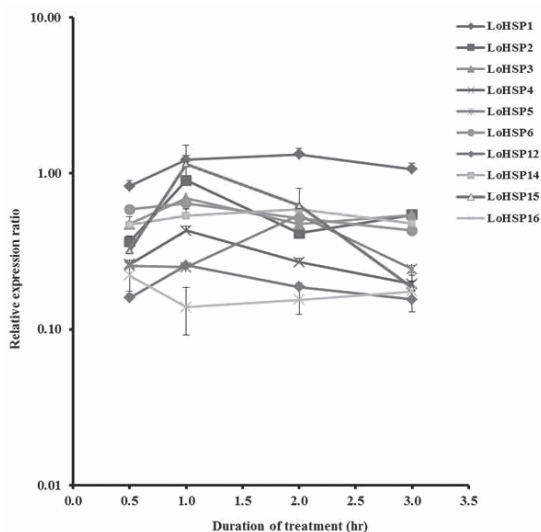
Fig. 1. Relative expression of L. oryophilus small Hsps under cold stress ( 0^{\circ}\text{C} ) compared to non-stressed controls. A colored version of this figure can be found in supplementary material for this article in Florida Entomologist 97(2) (June 2014) online at http://purl.fcla.edu/fcla/entomologist/browse
