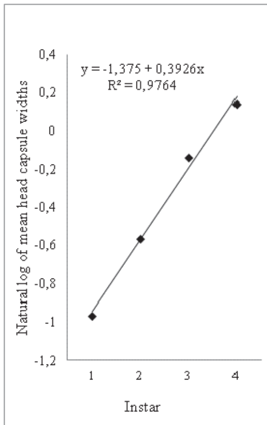
Fig. 2. Linear regression relationship between the natural logarithm of the mean larval head capsule widths and the number of the instars in the development of Rhysomatus subtilis larvae.
