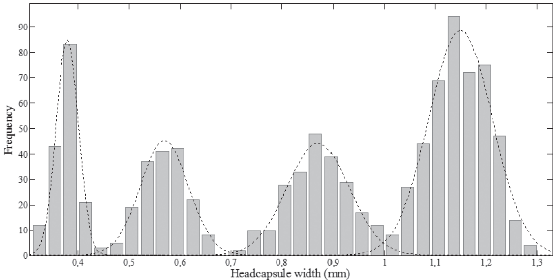
Fig. 1. Frequency distribution of observed head capsule widths (mm) of Rhysomatus subtilis larvae. Graphs were produced by the Hcap program.
