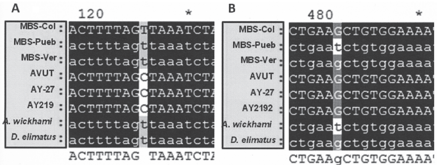
Fig. 7. Single nucleotide polymorphism of cpn60 UT sequences amplified from Dalbulus elimatus and Idiodonus wickhami compared with the 16SrI-B strains maize bushy stunt-Col (AB599712), maize bushy stunt-Pueb (KT444672), maize bushy stunt-Ver (KT444673), AVUT (AB599686), AY-27 (AB599688), and AY2192 (AB599687). (A) Similarities between the maize bushy stunt strains and the sequences obtained from the leafhoppers. (B) Similarity between maize bushy stunt-Pueb and the phytoplasma detected associated with Idiodonus wickhami and similarity between maize bushy stunt-Col and maize bushy stunt-Ver with the phytoplasma associated with Dalbulus elimatus , based on SNP in cpn60 UT sequences.
