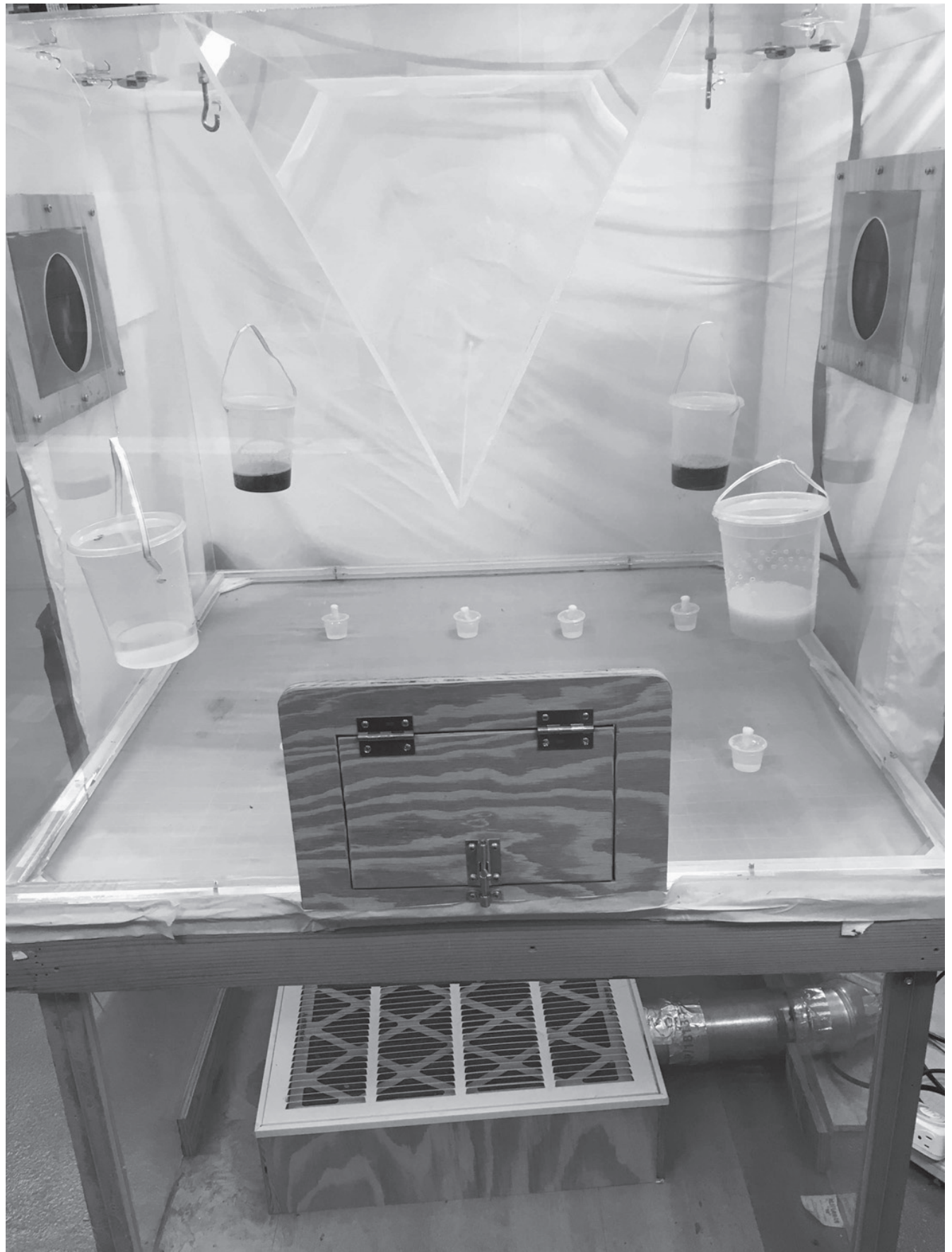
Fig. 1. The laboratory assay conducted in a wind chamber testing the effectiveness of baits to attract Drosophila suzukii .
