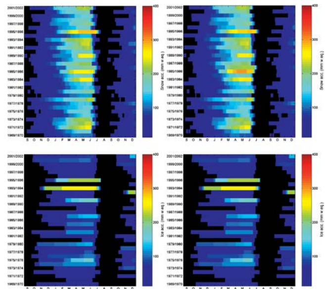
FIGURE 8. Raster plot of simulated winter snowpack (upper plots) and ground-ice thicknesses lower plots). Plots on left are for best-guess SBG and IBG (left panels) and on the right for the average of the 300 best simulations.
