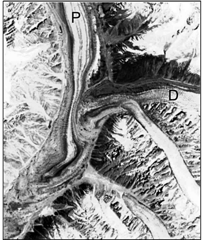
FIGURE 2. (a) Medial moraine loops at Susitna Glacier, Alaska; an excellent example of contorted moraine resulting from glacier surging (source: Online Glacier Photograph Database, Boulder, CO: National Snow and Ice Data Center/World Data Center for Glaciology). (b) Evidence of surge activity at the confluence of the Panmah (labeled P) and Drenmang (D) glaciers, Karakoram Himalaya (source: Landsat ETM+, viewed in panchromatic band 8). From this image the Drenmang glacier was coded as “2” in the inventory (strong morphological evidence of surging).
