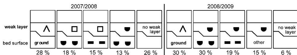
FIGURE 10. Relative amount of weak layer–bed surface combinations observed in the snowpack for the snow seasons 2007/2008 (5 snow pits on the left) and 2008/2009 (5 snow pits on the right). Grain shape symbols are explained in Figure 7.
