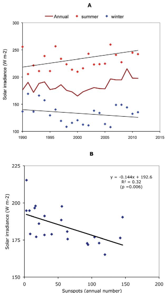
FIGURE 7. (A) Trends in surface solar irradiance in the Snowy Mountains above the treeline (>1700 m). (B) Relationship of the annual solar irradiance with the average number of sunspots per year.
