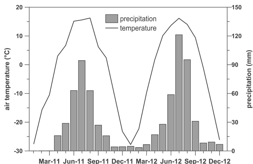
FIGURE 3. Monthly air temperature ( ^{\circ}\text{C} ) and precipitation (mm) values measured at the lower steppe site from January 2011 until December 2012.
