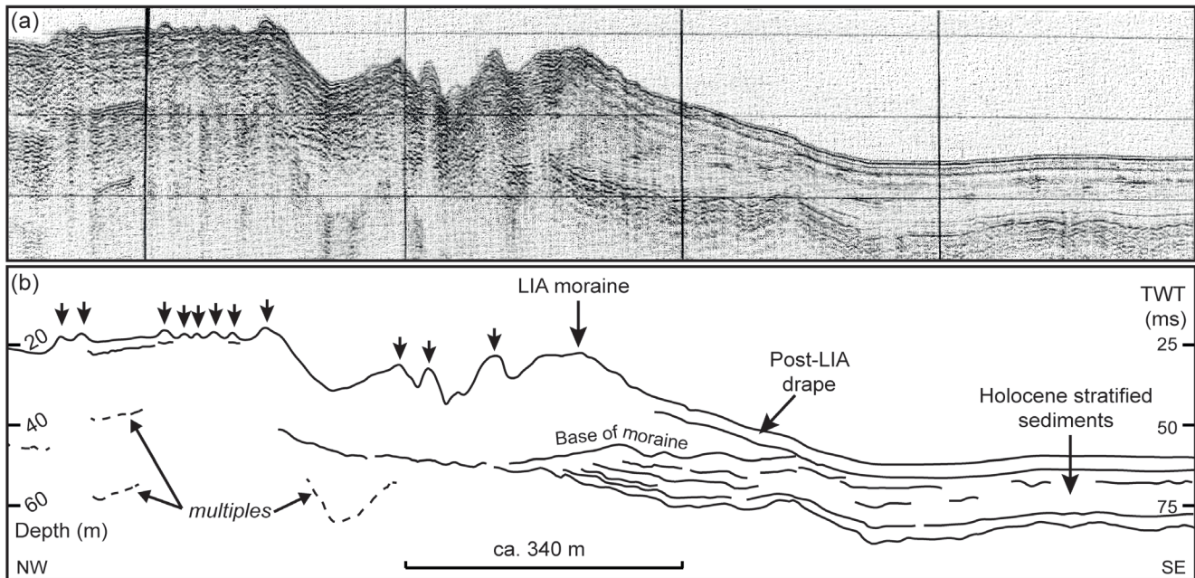
FIGURE 3. (a) Boomer seismic profile showing small transverse moraines and a larger, terminal moraine assumed to be from the Little Ice Age (LIA) in the gap between bathymetric data sets. (b) Interpretation of the seismic profile in panel (a). Vertical arrows are small transverse ridges. Profile located on Figure 2 and adapted from Whittington et al. (1997).
