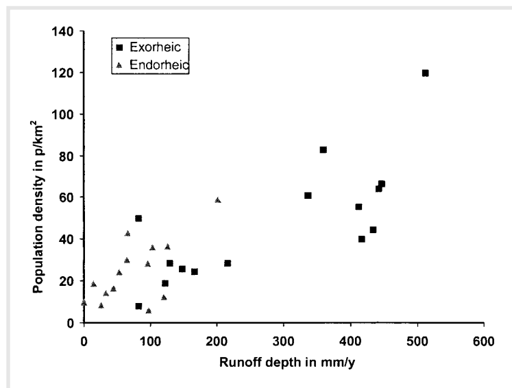
FIGURE 4 Population density ( p/\text{km}^2 ) versus runoff depth in exorheic (■) and endorheic (▲) regions for 15 relief classes ( 30' resolution).
