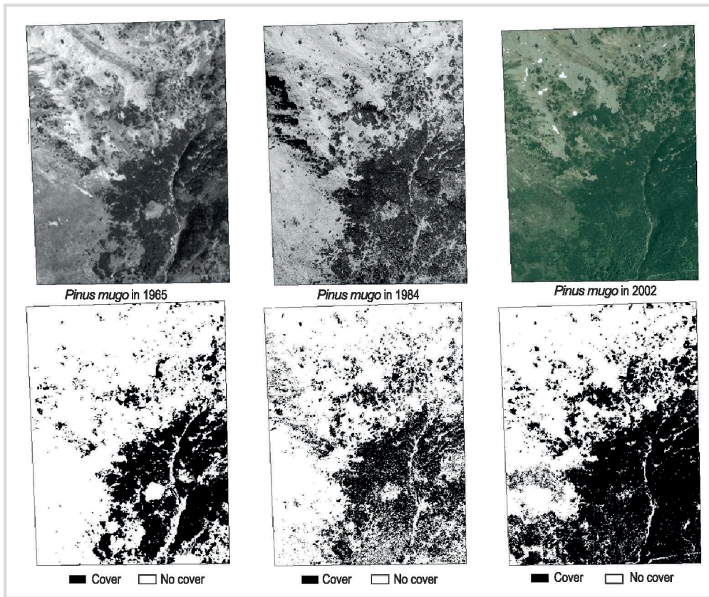
FIGURE 2 Example of the comparison between aerial photographs: changes between 1965, 1986, and 2002 in 1 analyzed valley (locality 1, Banikov valley; Figure 1).
