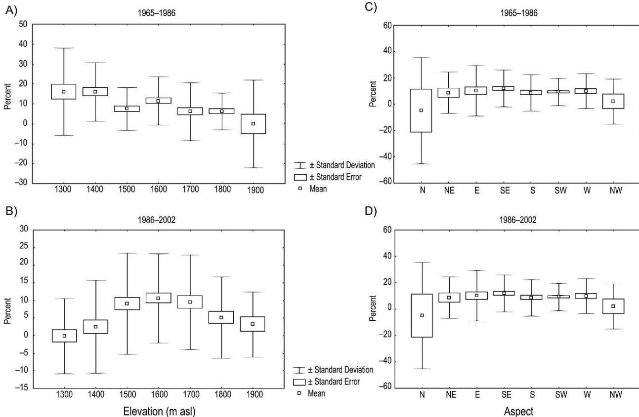
FIGURE 4 Increments in dwarf pine cover in the western Tatra Mountains in the periods 1965–1986 and 1986–2002, according to (A and B) elevation and (C and D) aspect. In the earlier period, the groups did not differ according to aspect. (C) Kruskal–Wallis nonparametric test at p = 0.05 . (D) In the period 1986–2002, the following aspects differed significantly: N:NE, N:SW, NE:W, NE:S, NE:SE, SE:SW, S:SW, and SW:W.
